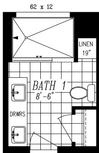
OPT. 48x72 SHWR. W/ DBL LAV
